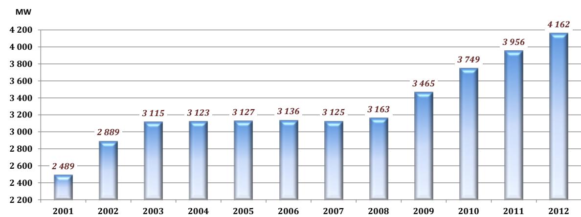
Figure 5-1: Cumulative Wind Installation (MW) of Denmark
