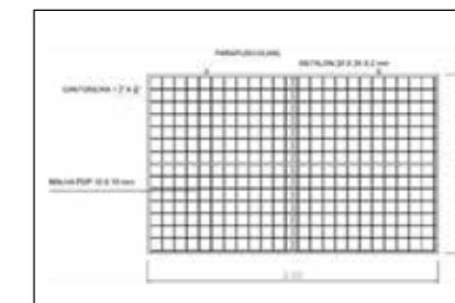
Porta guilhotina
